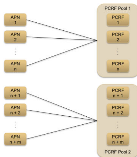
Figure 2-56 Relationship between APNs and PCRF Pools
